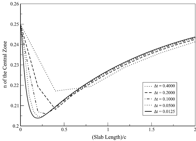
Fig. 3. Transient behavior of n(t) – the fraction of atoms in the excited state – in the central zone for the semi-implicit difference method.
