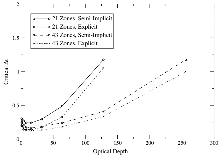
Fig. 8. Graphs of the time step size versus optical depth of the slab near the edge of numerical stability for the explicit and semi-implicit difference methods. Two zone thicknesses are shown. The vertical axis is in units of (slab length)/ c . Instability for a given treatment of the source terms occurs above the line. Beyond the termination of the lines, the calculations are stable for any time step.
