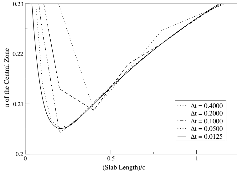
Fig. 2. Detail of the transient behavior of n(t) – the fraction of atoms in the excited state – in the central zone for the explicit difference method.
