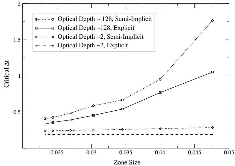
Fig. 9. Graphs of the time step size versus zone size near the edge of stability for the explicit and semi-implicit difference methods. The slabs are divided into zones of uniform size and two optical depths for each scheme are shown. The vertical axis is in units of (slab length)/ c , and the horizontal axis is in fractions of the total length of the unit slab.
