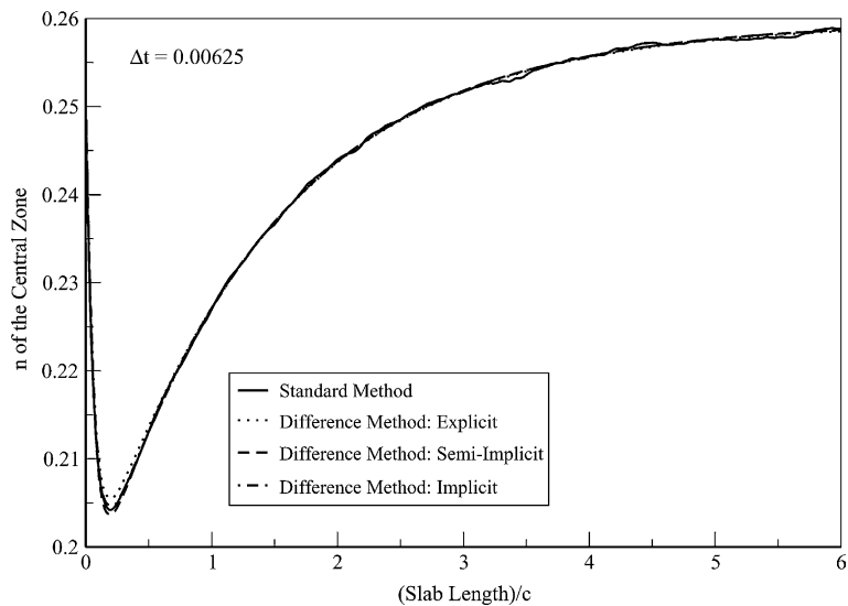
Fig. 7. Transient behavior of n – the fraction of atoms in the excited state – of the three difference methods and the standard method.
