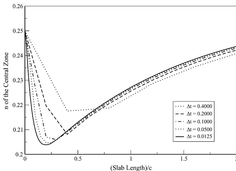
Fig. 4. Transient behavior of n(t) – the fraction of atoms in the excited state – in the central zone for the implicit difference method.
