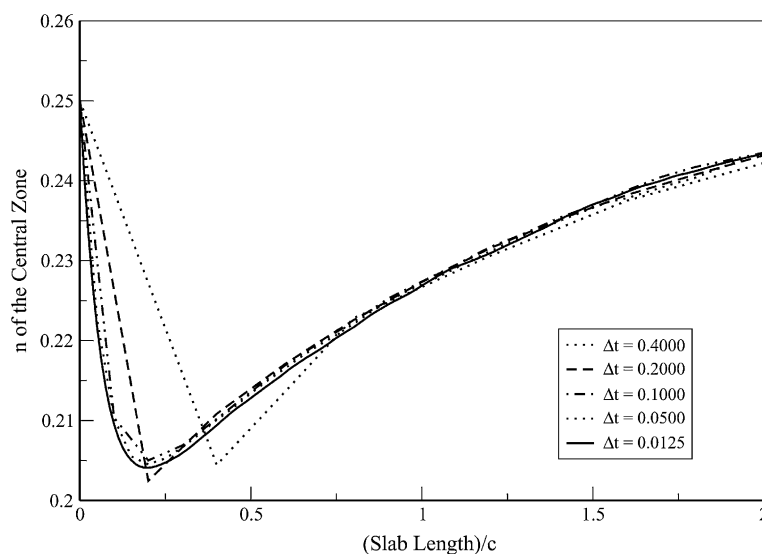
Fig. 5. Transient behavior of n(t) – the fraction of atoms in the excited state – in the central zone for the standard method.
