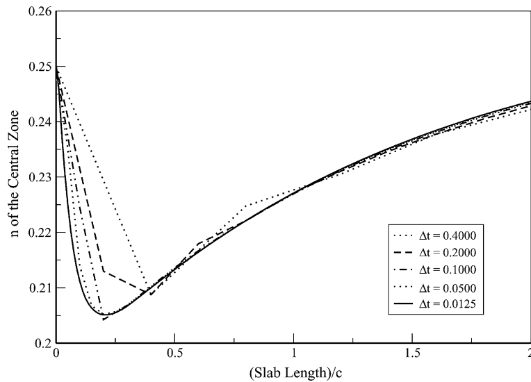
Fig. 1. Transient behavior of n(t) – the fraction of atoms in the excited state – in the central zone for the explicit difference method.
