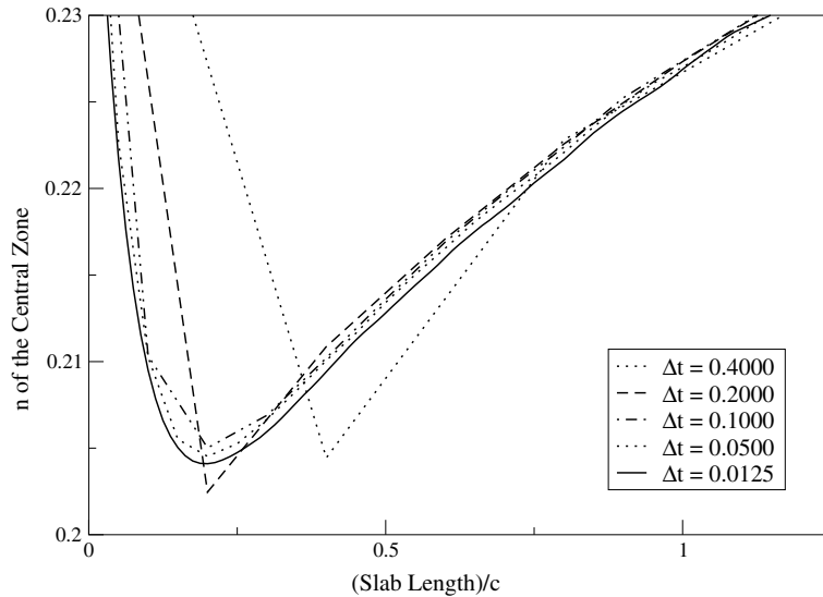
Fig. 6. Detail of the transient behavior of n(t) – the fraction of atoms in the excited state – in the central zone for the standard method.
